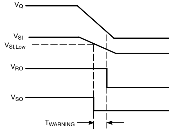
Figure 20. SO Warning Timing Waveform
