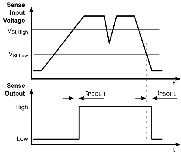
Figure 21. Sense Timing Diagram
